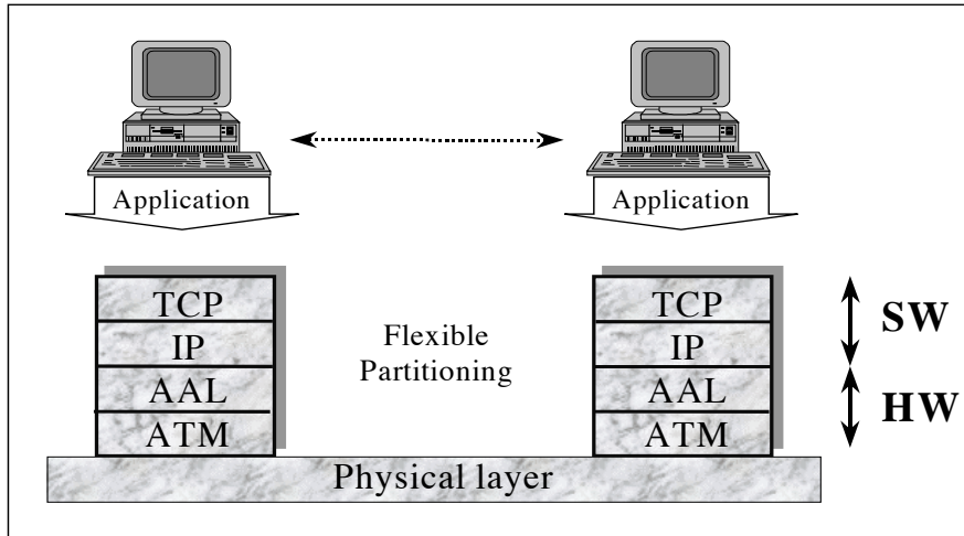
Figure 1. Applications connected to the network via NICs.
