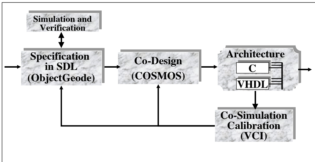
Figure 5. Design flow adopted for the architecture exploration of the NIC system.
