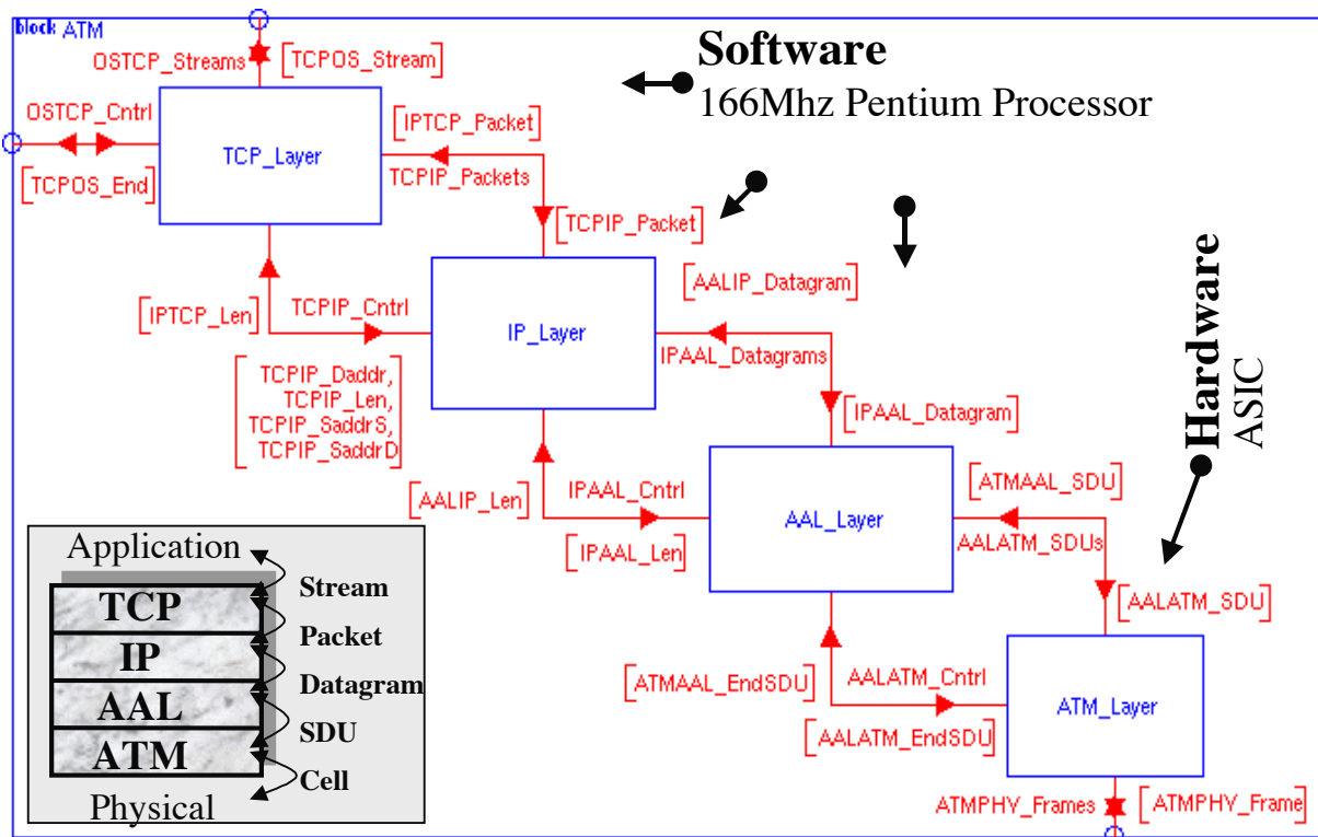
Figure 3. Structure of the NIC system described in SDL.
