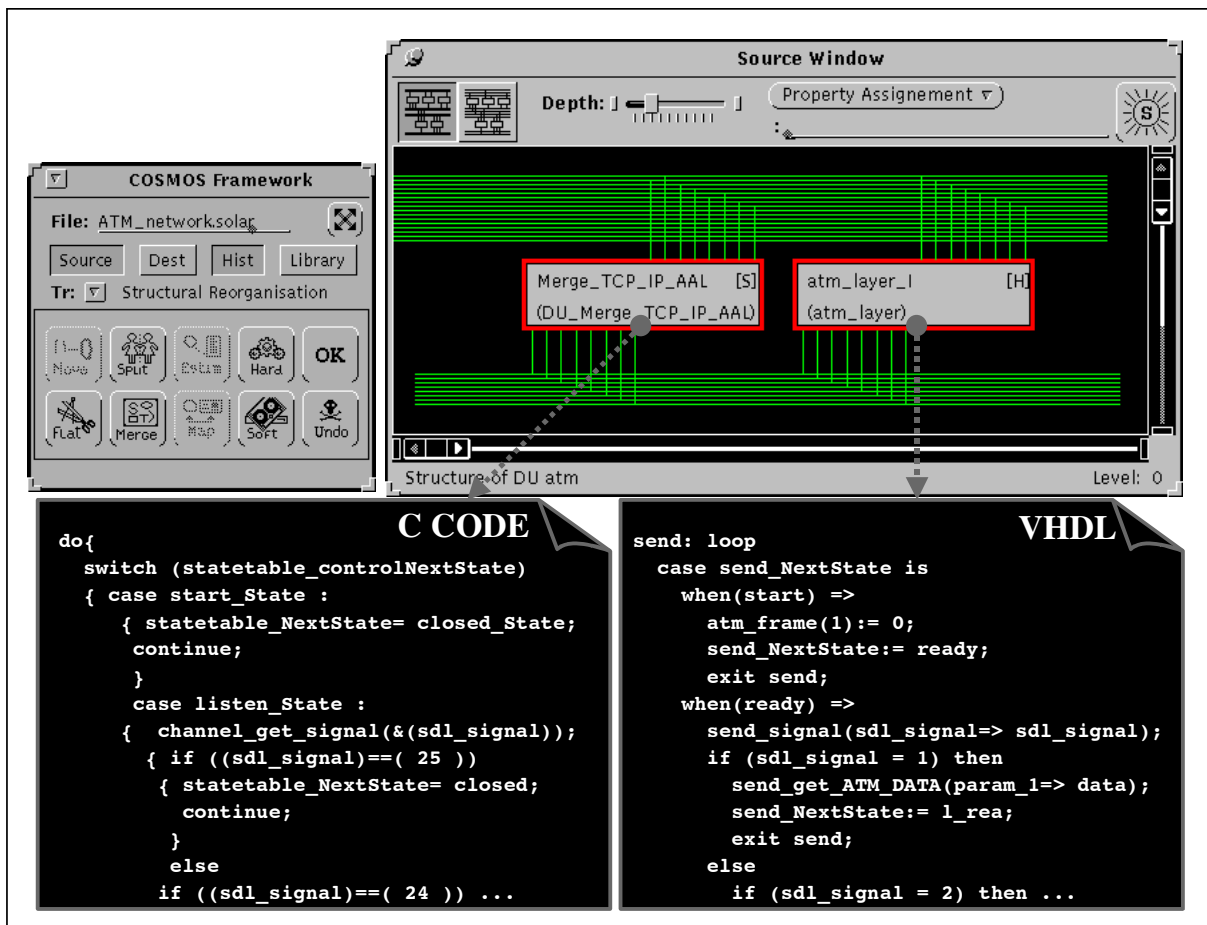
Figure 7. The produced C/VHDL model in Cosmos
