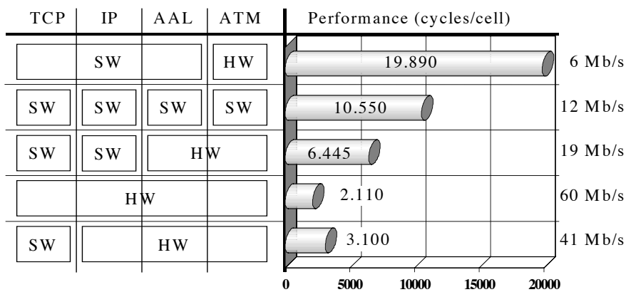
Figure 8. Performance of different ATM NIC implementations.
